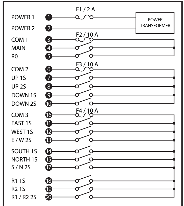
Q808 Wiring diagram
