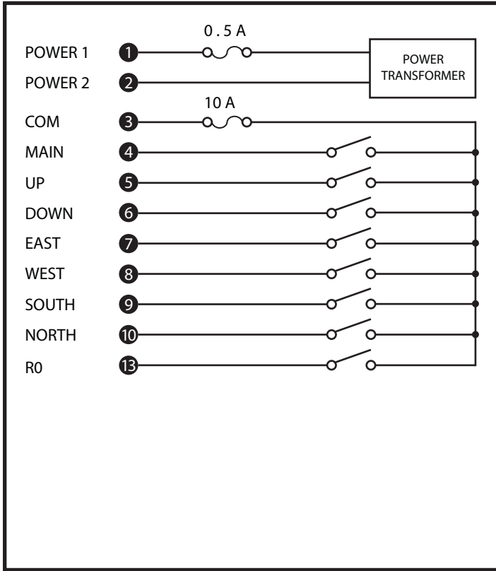
Q800 Wiring diagram
