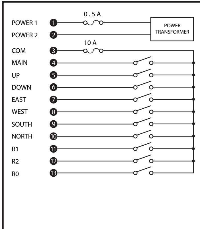
Q800 Wiring diagram
